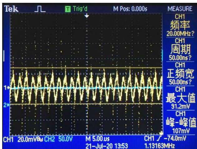
Noise ( V_{IN} = 57V , I_O = 1.25A , 5 ~ 20MHz bandwidth)
