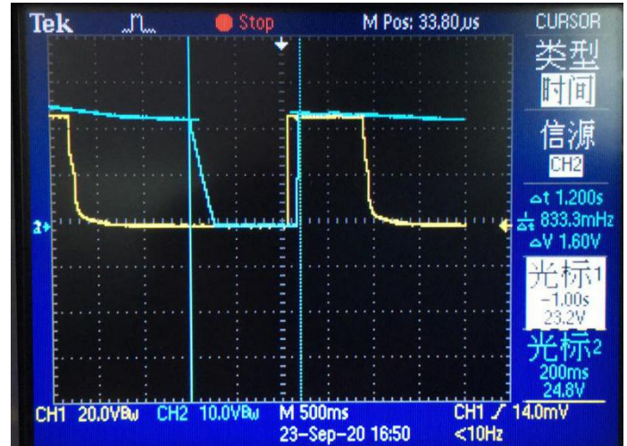
Output response & load (24V / 0.6A)
