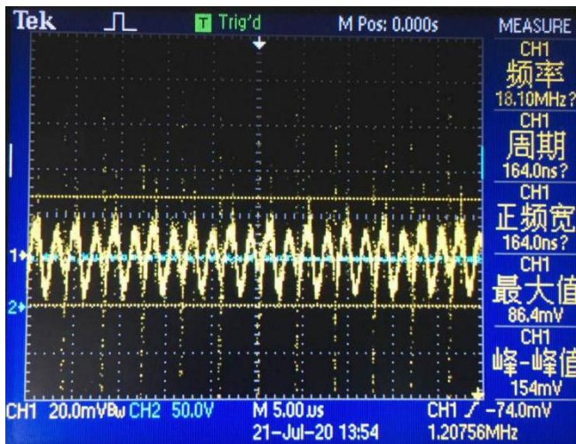
Noise ( V_{IN} = 48V , I_O = 1.25A , 5 ~ 20MHz bandwidth)
